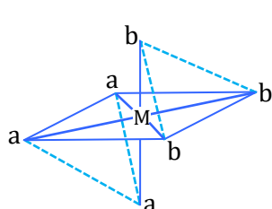
Facial (fac) Optically inactive
